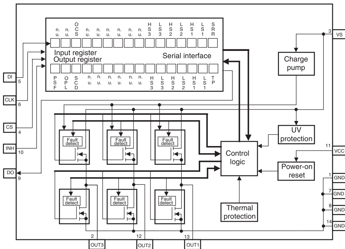
Figure 1-1. Block Diagram
